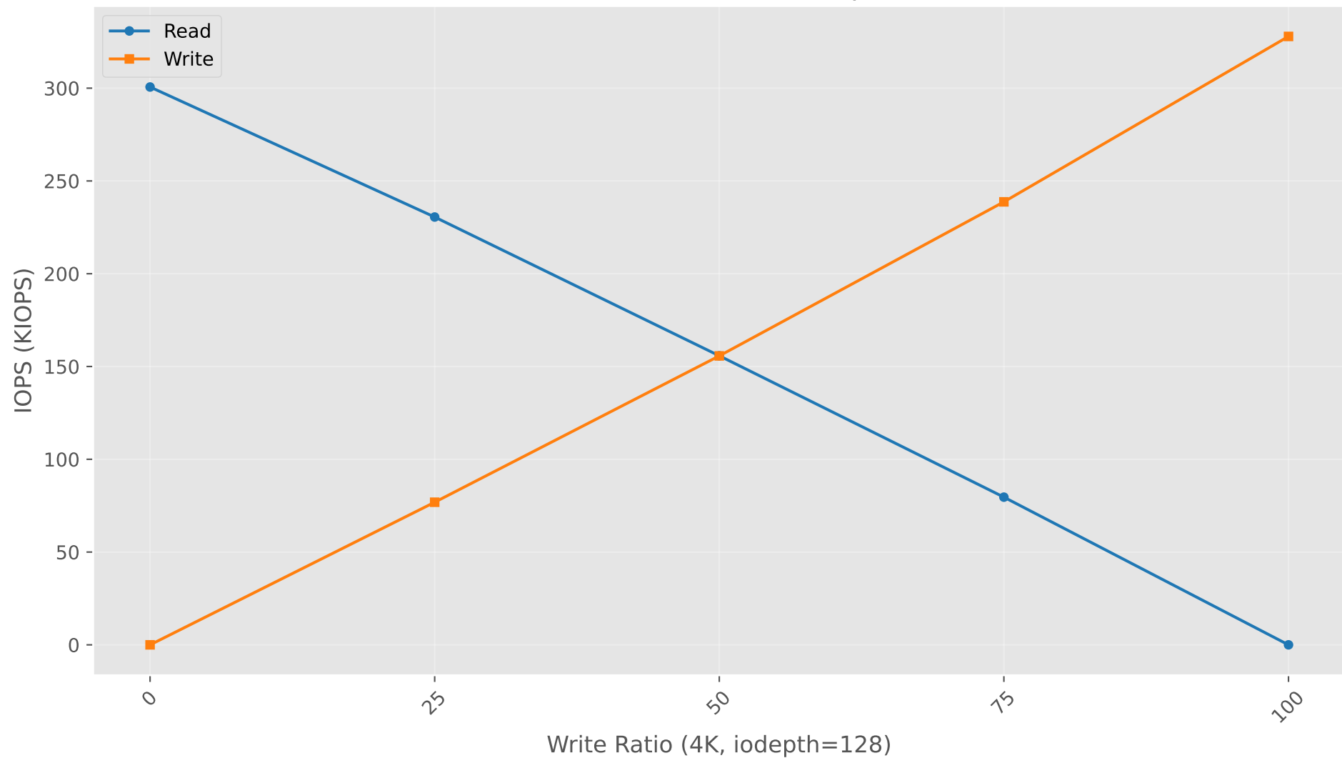
IOPS vs Write Ratio (4K, iodepth=128)
